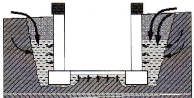
Fig. 2 Ground water distribution
