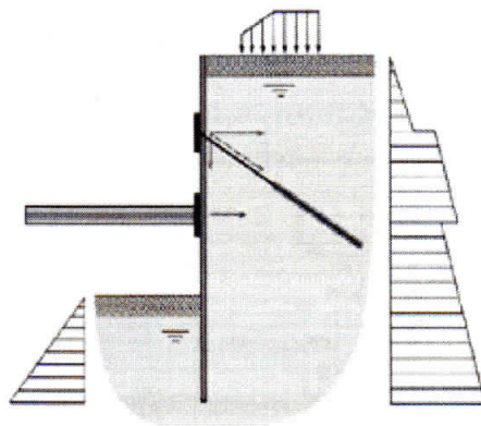
Fig. 5. Design scheme
