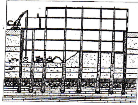
Fig. 3. Construction of underground structures
