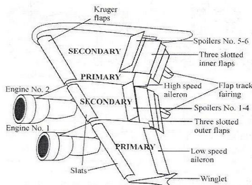
Fig. 2. Large transport aircraft: typical control surfaces.
