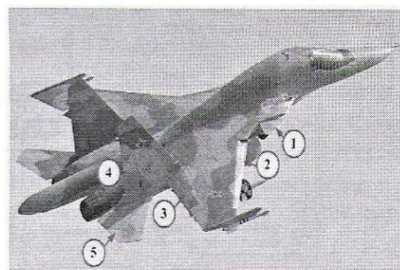
Fig. 3. SU-34 flight control surfaces scheme: 1 are two consoles canards; 2 are two sections rotary wing socks; 3 are two sections flaperons; 4 are two sections rudder; 5 are two consoles horizontal tail.
