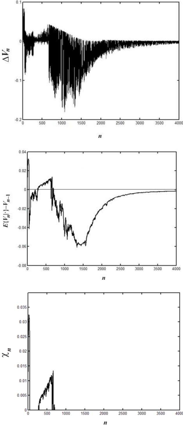
Figure 6. Variables \Delta V_n , E\{V_n\} - V_{n-1} and \chi_n in Example 3.
